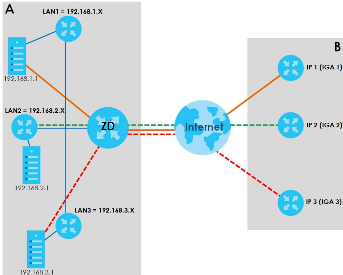
Figure 184 NAT Application With IP Alias
