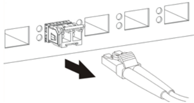
Figure 50 Opening the Transceiver's Latch Example
