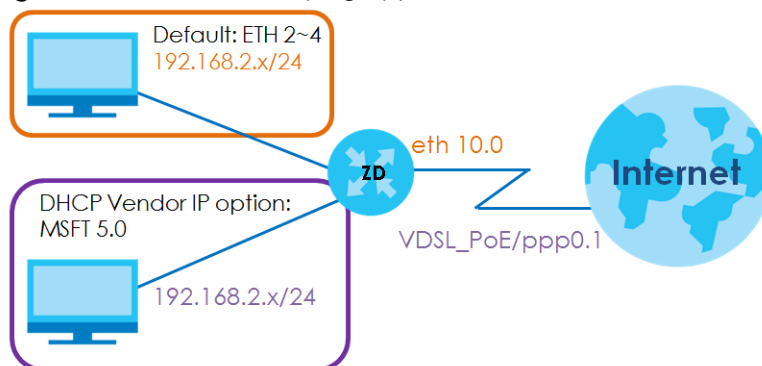
Figure 192 Interface Grouping Application
