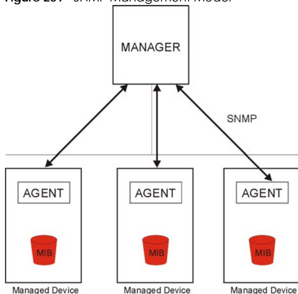
Figure 259 SNMP Management Model
