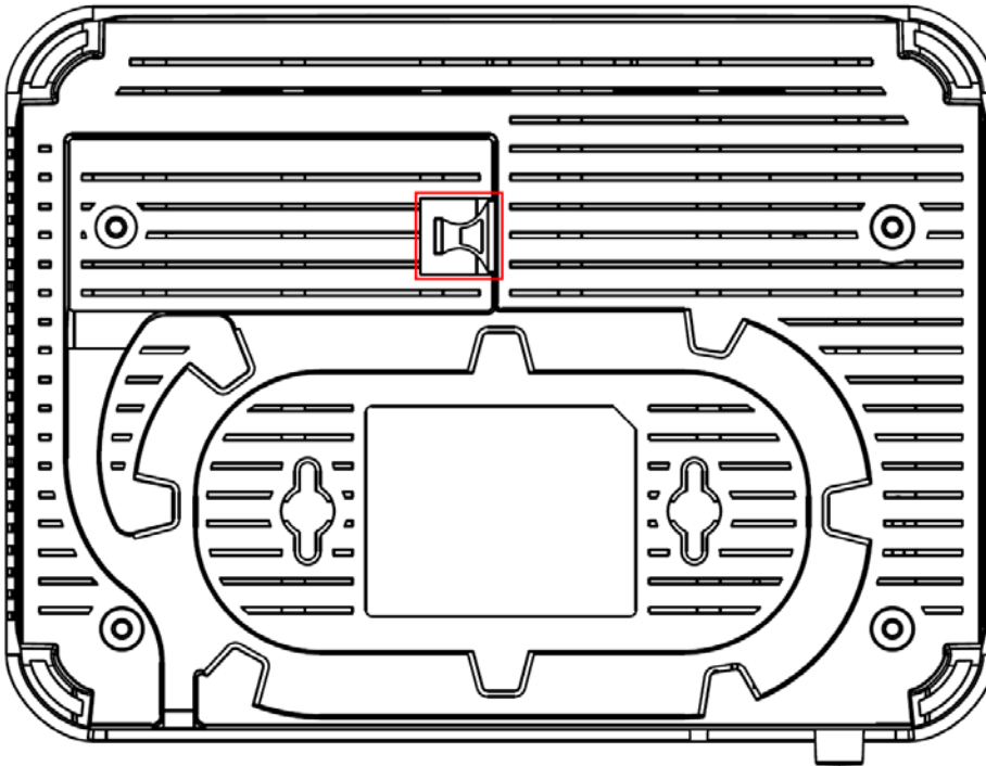
Figure 44 PX5301-T0 Bottom Panel (PON Port)
