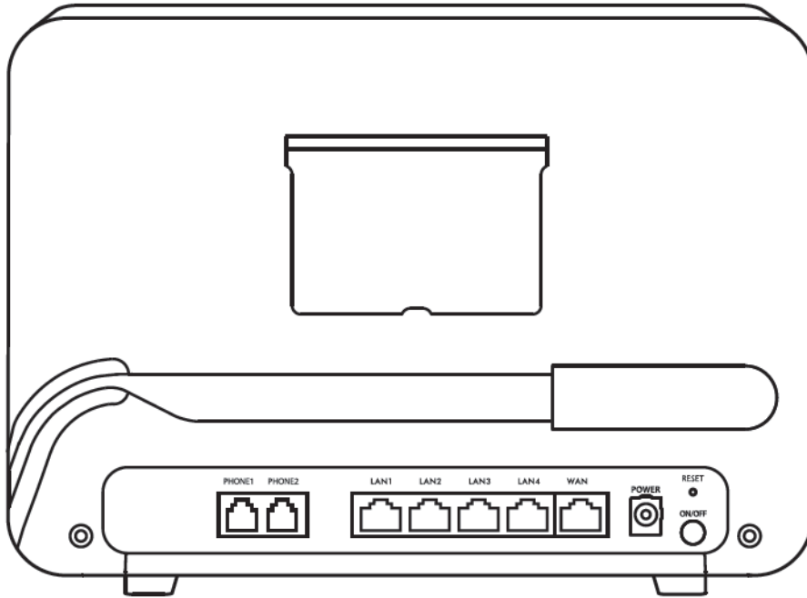
Figure 31 EX5401-B0 / EX5401-B1
