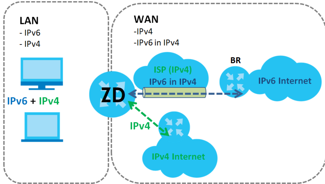
Figure 95 IPv6 Rapid Deployment
