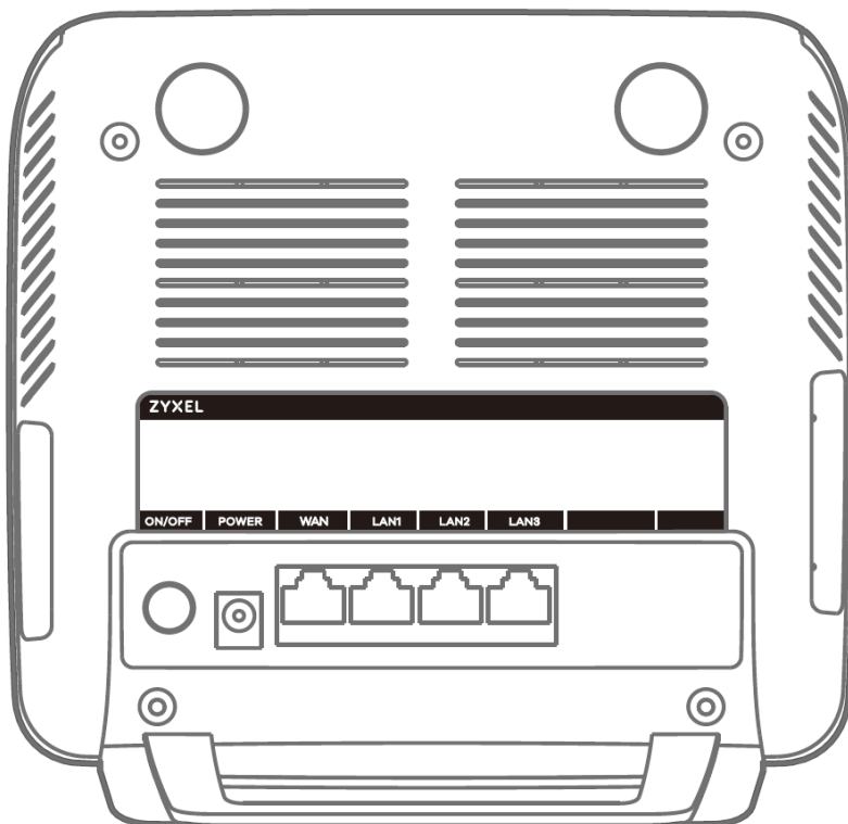
Figure 34 EX3500-T0
