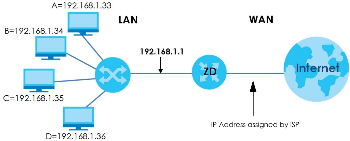
Figure 185 Multiple Servers Behind NAT Example
